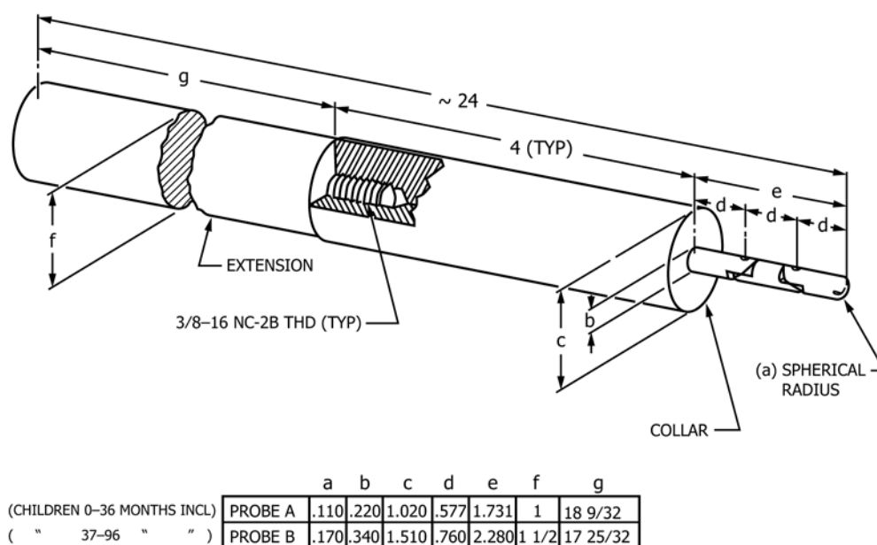
FIG. 1 Accessibility Probes
